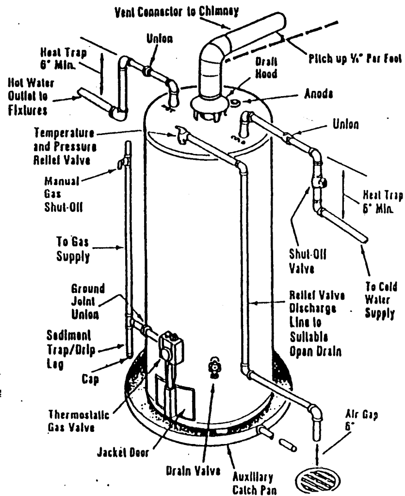
Fig. 4 — Typical Installation
